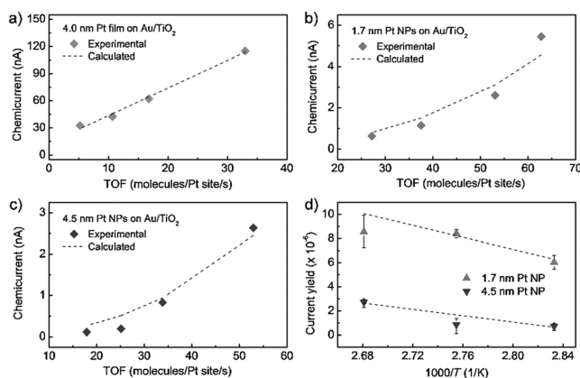
Figure 4. Chemicurrent from the Au/TiO 2 nanodiodes with a) 4 nm thick continuous Pt film, b) 1.7, or c) 4.5 nm Pt NPs, plotted as a function of the TOF for H 2 oxidation. d) Comparison of chemicurrent yield during reaction with 1.7 or 4.5 nm Pt NPs.
